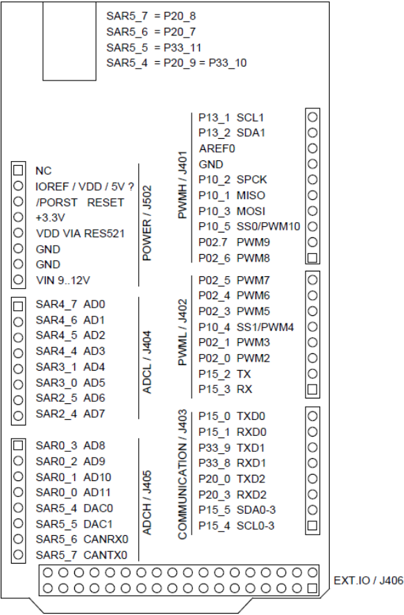
Figure 7 TC275 to Arduino Connector Mapping
