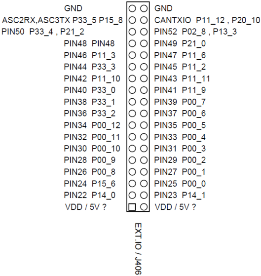
Figure 8 TC275 to Arduino EXT IO Connector Mapping
