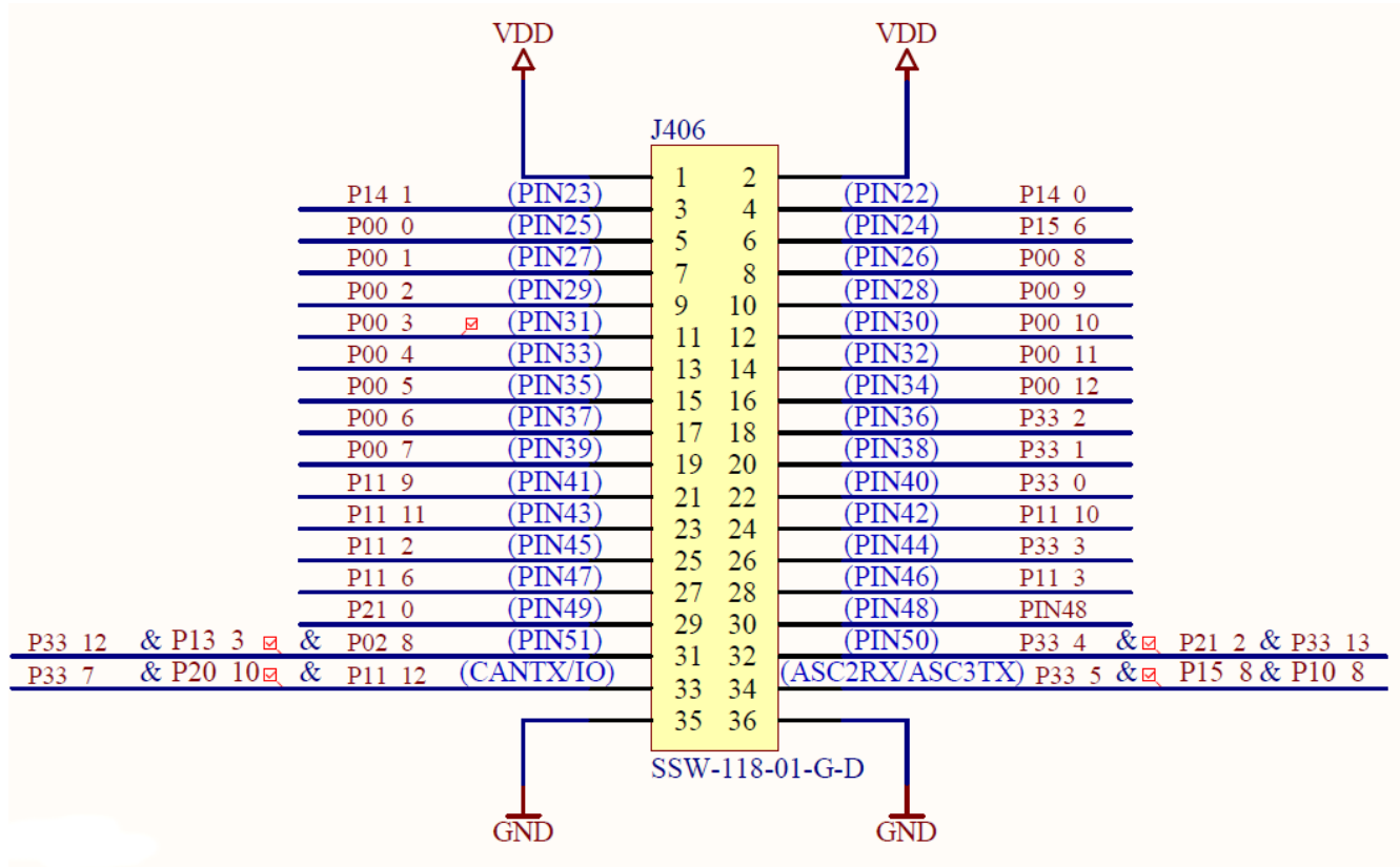
Figure 5 Extended IO Connector
